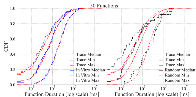
Figure 2: Distribution validation of function durations between workload samples from our method and random selection against the original Azure trace. Both samples contain 50 functions. Our method approximates well the tail distributions of the 78K functions of original trace with only 50 functions.
