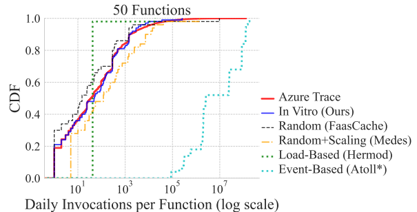
Figure 1: Distribution comparison of daily invocations per function of workload models from prior works (FaasCache [18], Medes [46], Atoll [48], and Hermod [24]) with our workload model (§2.2). For fairness, all workload models are scaled to 50 functions (see §2.1). *Atoll scales the invocations based on their testbed but does not specify the scales, so we do not do such scaling here.
